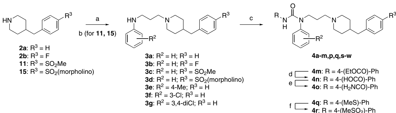
Scheme 1. Reagents: (a) acrolein, cat. DBU, THF, then R 2 -PhNH 2 , NaBH(OAc) 3 ; (b) N -(3-chloropropyl)aniline hydrochloride, KI, K 2 CO 3 , MeCN, DMF; (c) R-NCO, Et 3 N, DCM; (d) aq NaOH, EtOH; (e) NH 4 Cl, Et 3 N, EDC, HOBt, DMF; (f) Oxone, aq H 2 SO 4 , MeOH.
